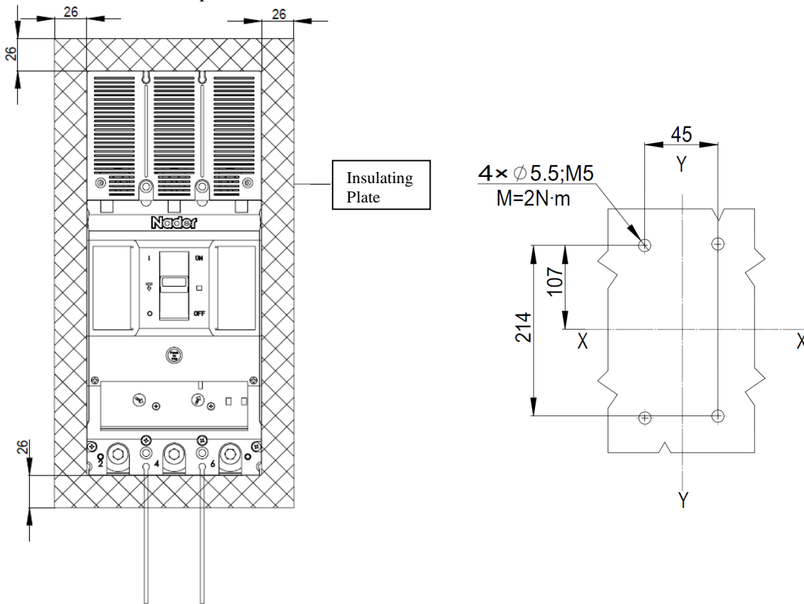
Insulating Plate Dimensions
