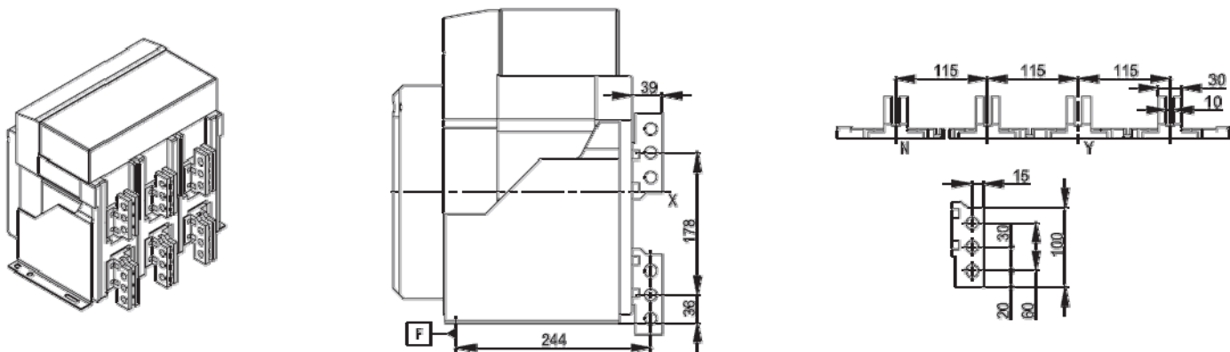
3200A、4000A Horizontal extended, Vertical extended
