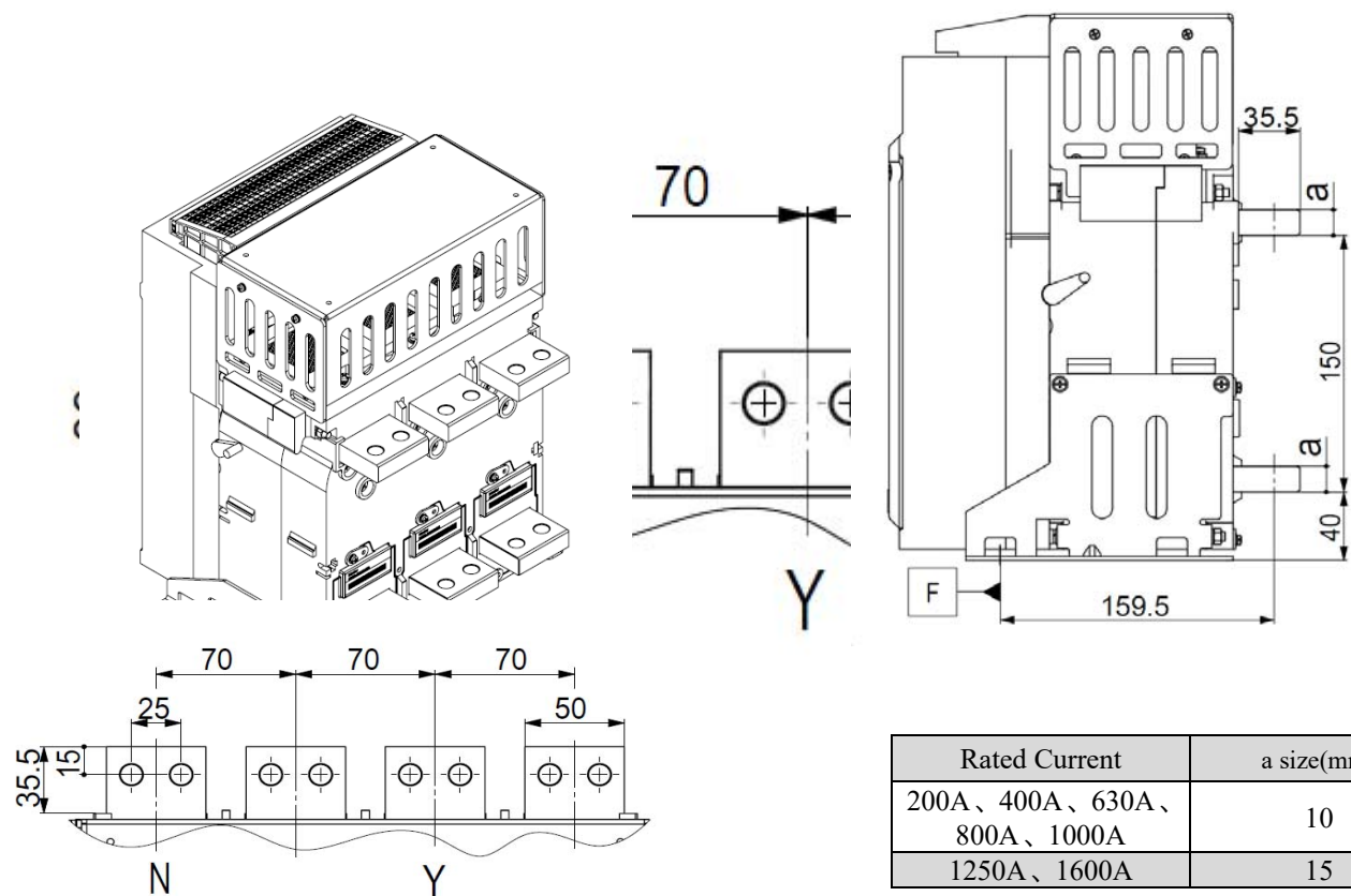
NDW2-1600 Fixed Type Vertical Wiring
