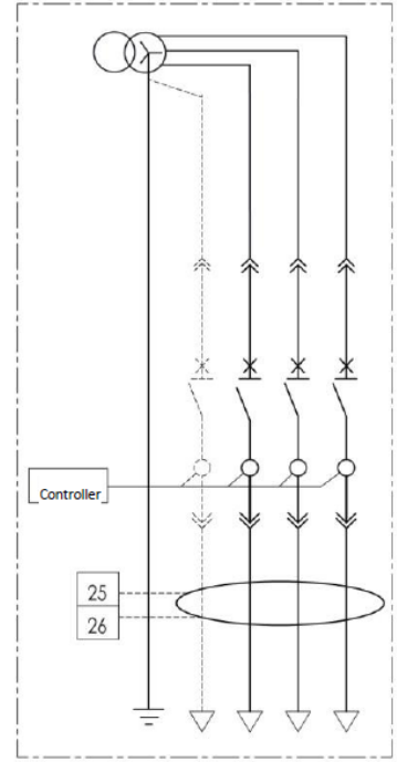
Leakage grounding protection
