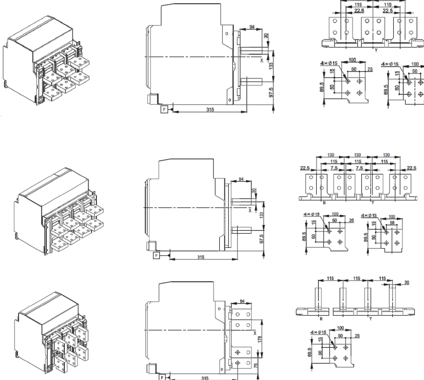
3200A, 4000A Horizontal extended, Vertical extended
