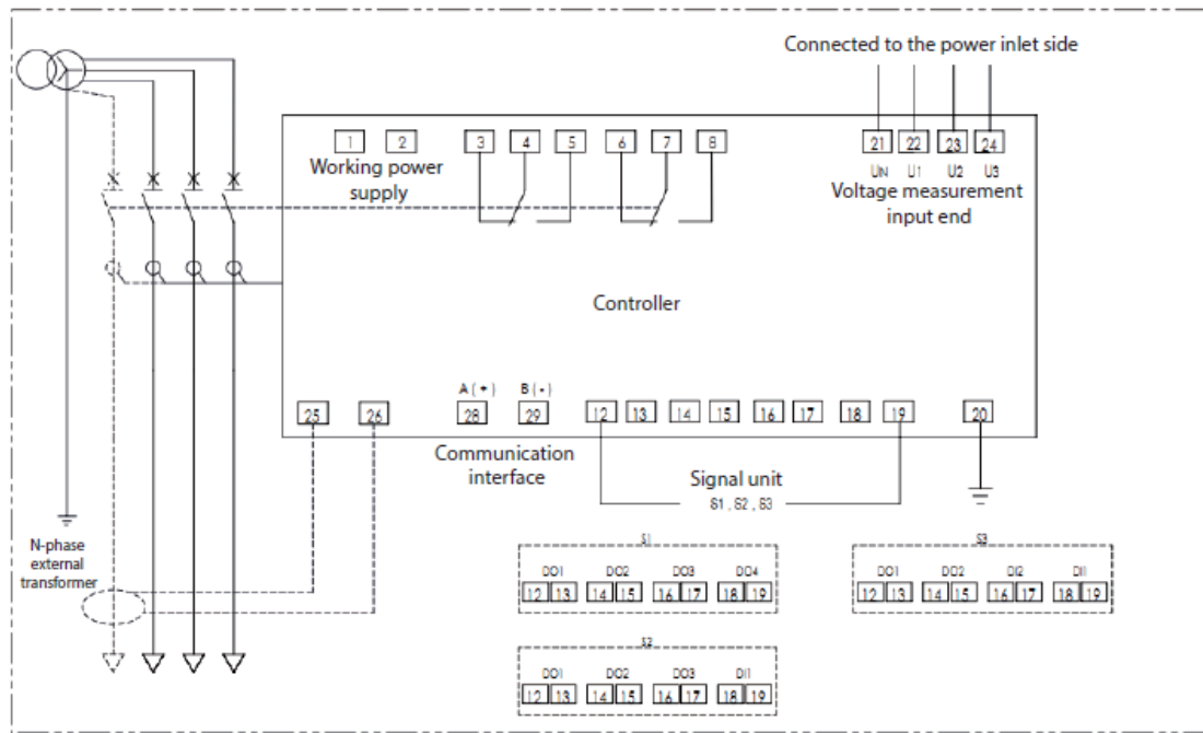
Controller input/output interface
