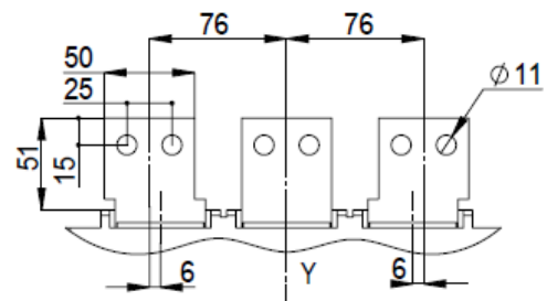
3 poles
