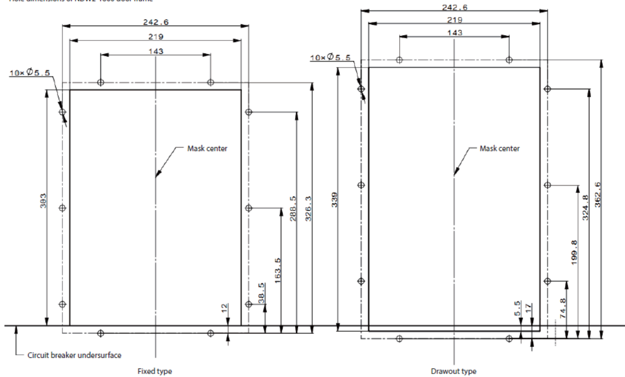
Hole dimensions of NDW2-1600 door frame
