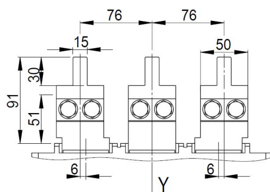
3 poles
