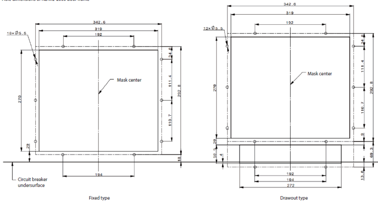
Hole dimensions of NDW2-2000 door frame
