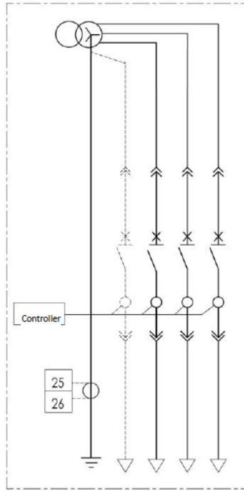
Ground current type grounding protection
