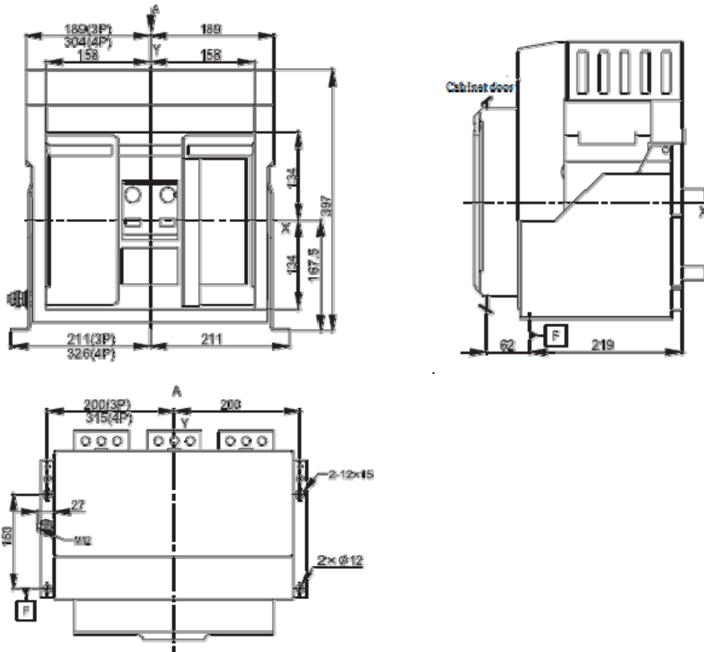
NDW2-3200 fixed type wiring
