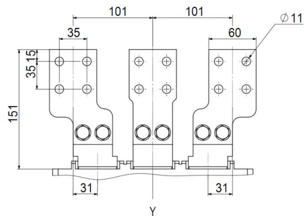
3 poles
