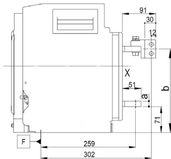
NDW2-1600 Drawer Type Hybrid Wiring (upper vertical lower horizontal wiring)
