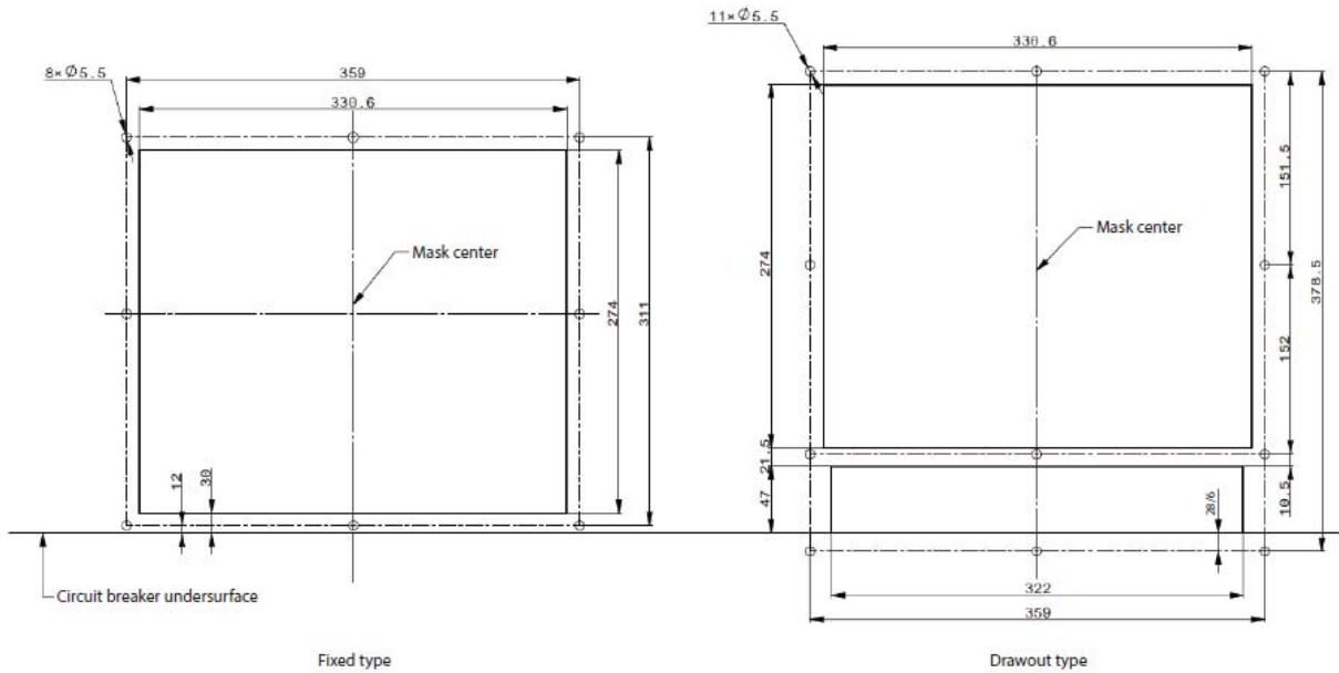
Hole dimensions of NDW2-3200/4000/6300 door frame
