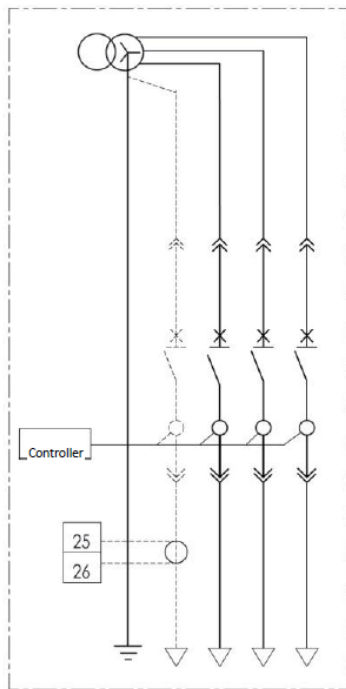
3-pole connecting N-phase difference type grounding protection
