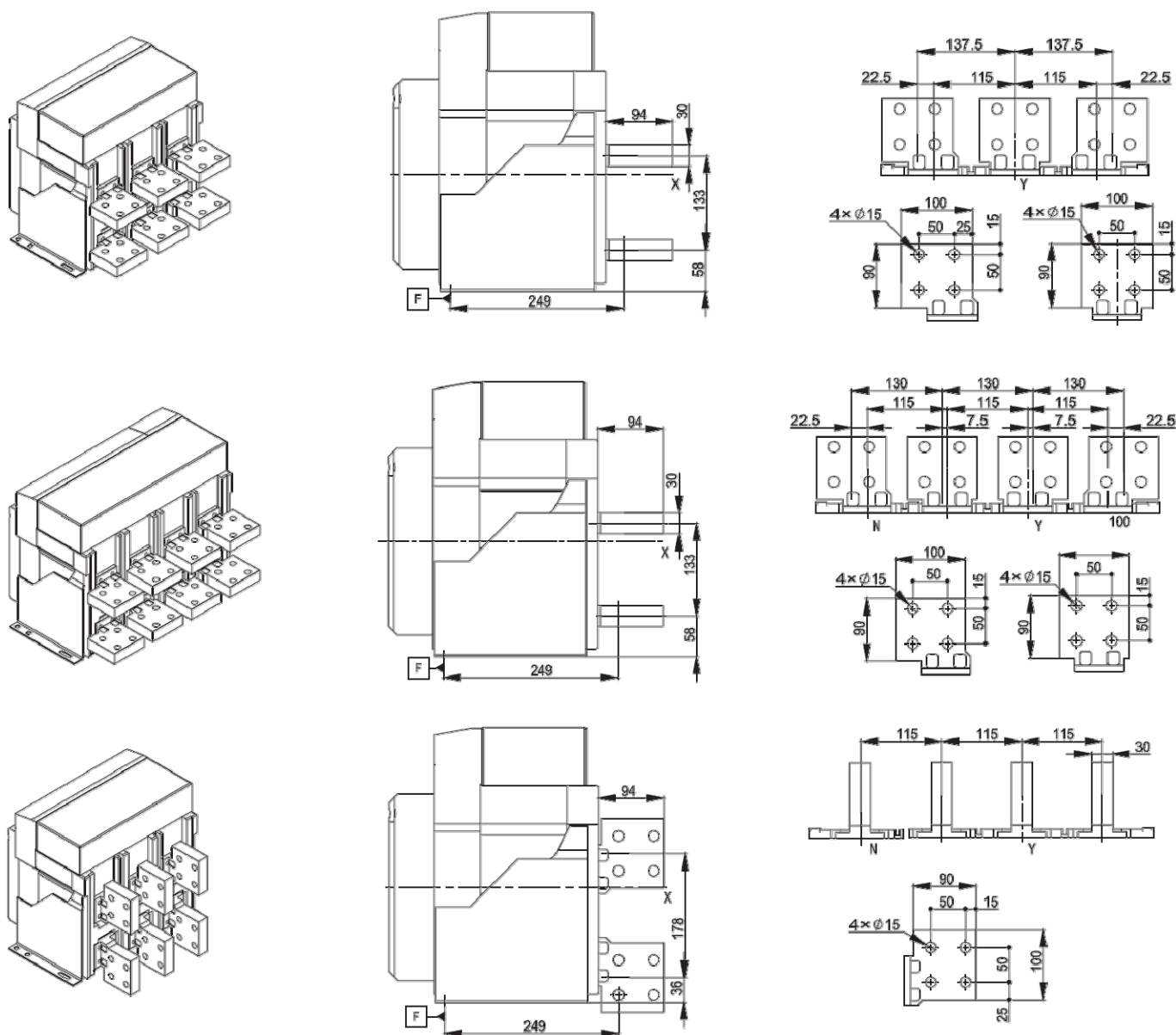
3200A、4000A Horizontal extended, Vertical extended
